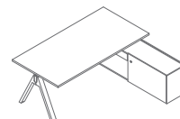
V04PM 2000 / 1800 / 740 120.22 kg
